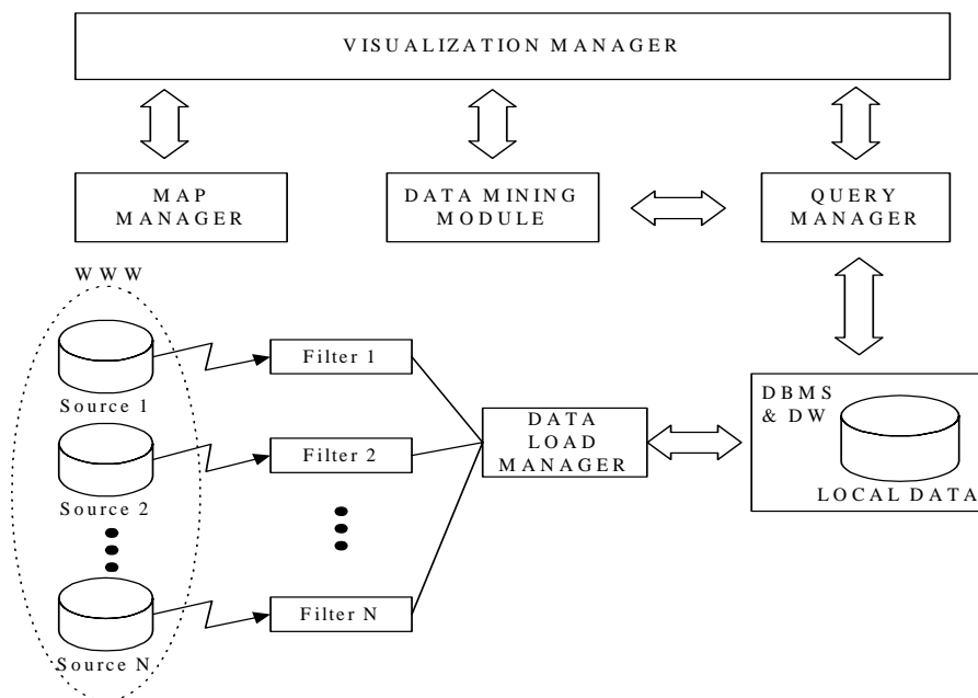
Figure 1. The SEISMO-SURFER architecture.
