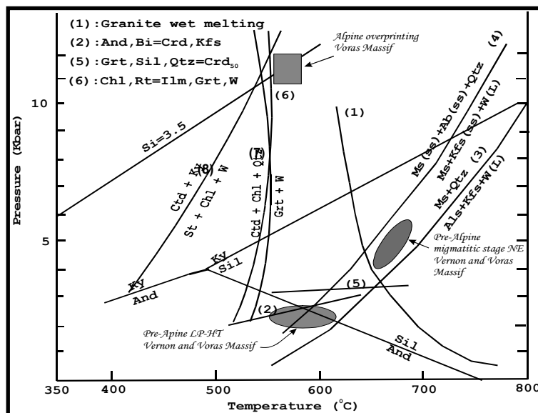
Fig. 5: P-T diagram with reaction curves in a pelitic system, taken from Spear (1995). Isoleth Si=3.5 is from Massonne and Schreyer (1987). Reaction curves 2 and 5 are taken from Mposkos et al., 2001; reaction curves 6, 7 and 8 are calculated with the TWEEQU software (Berman, 1991) using analyzed mineral composition.
