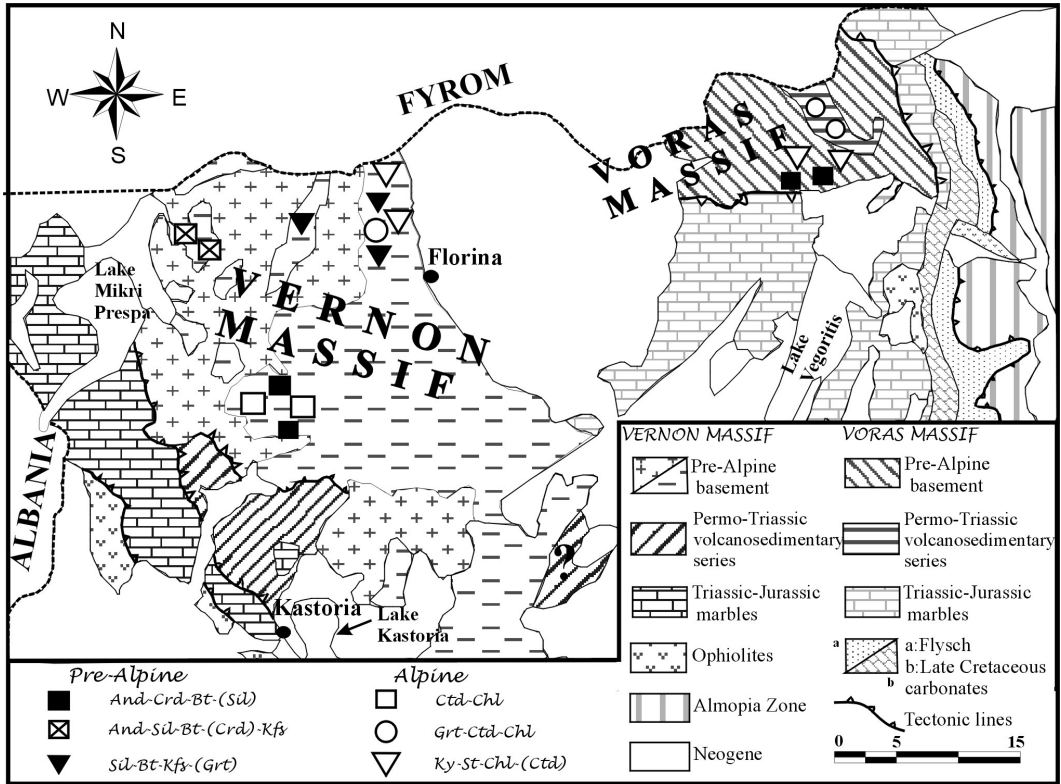
Fig. 1: Simplified geological map of the Voras and Vernon Massifs (after Kiliias and Mountrakis, 1989, and Avgerinas et al. 2003, modified).
