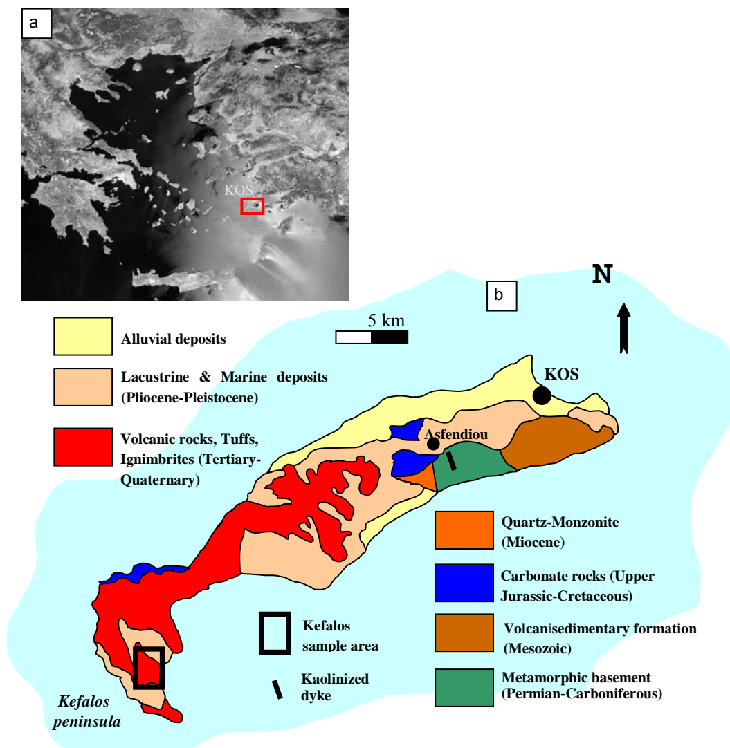
Figure 1. a). Geographic position of Kos Island, in the Southeastern Aegean Sea. b). Geological sketch map of Kos Island (after Triantaphyllis 1994, 1998).
